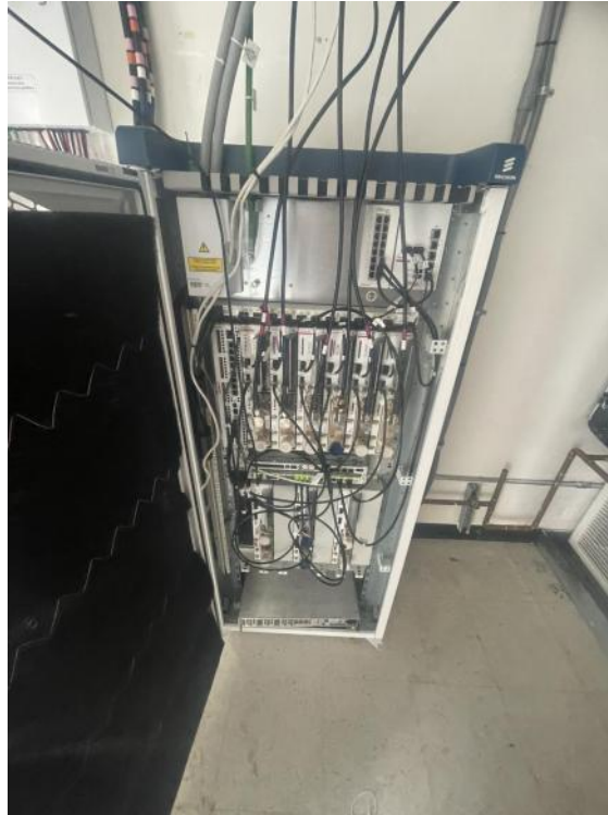
BTS Equipment Cabinet
